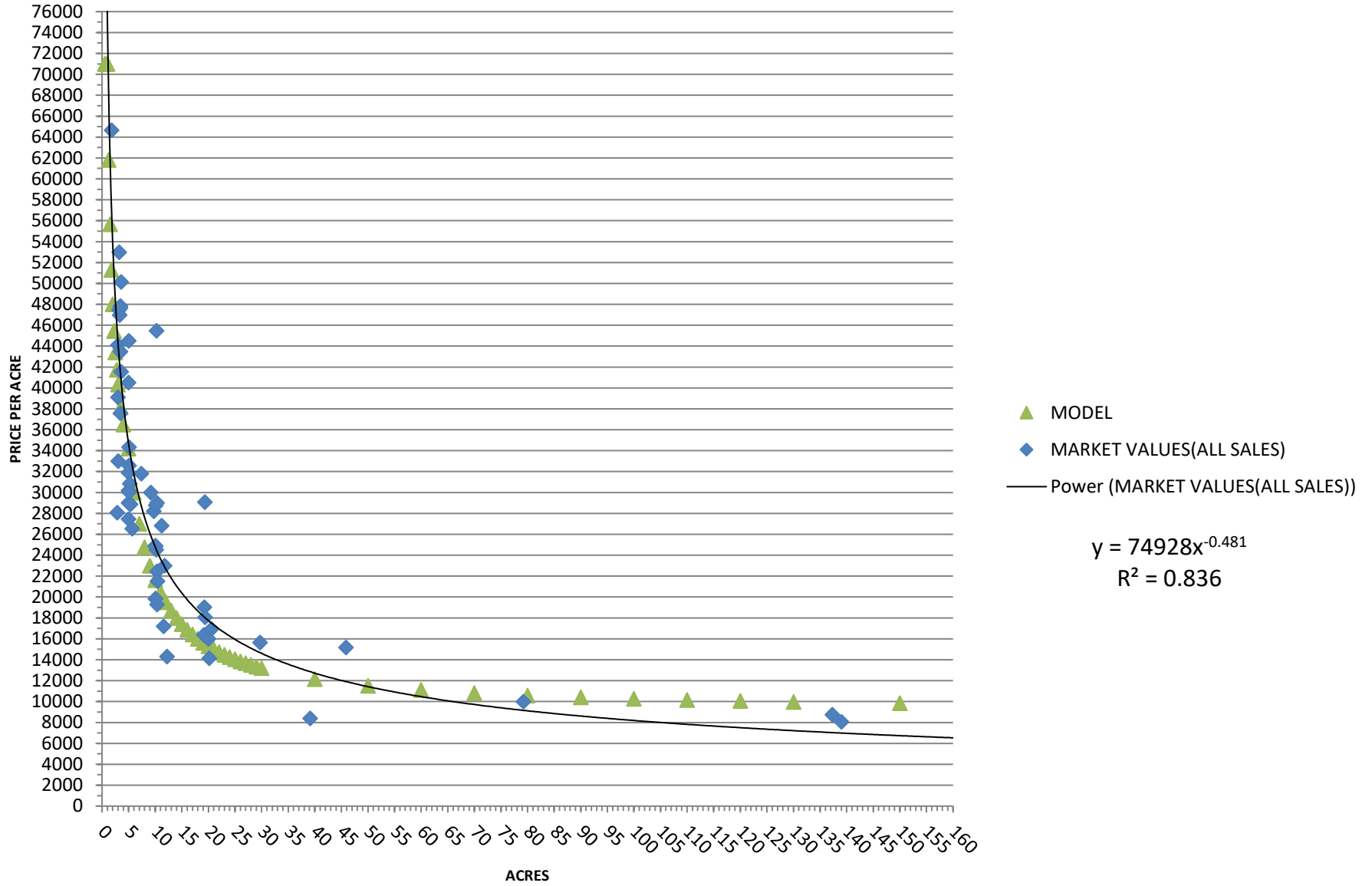
SCATTER GRAPH SHOWING RELATIONSHIP IN SELLING PRICE PER ACRE TO VALUATION MODEL PRICE PER ACRE ZERO TO 160 ACRES
